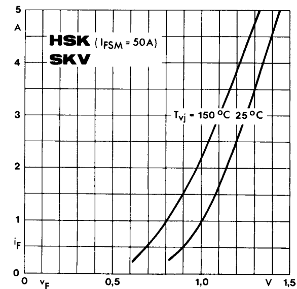
Fig. 5 a Forward characteristic of a single chip
