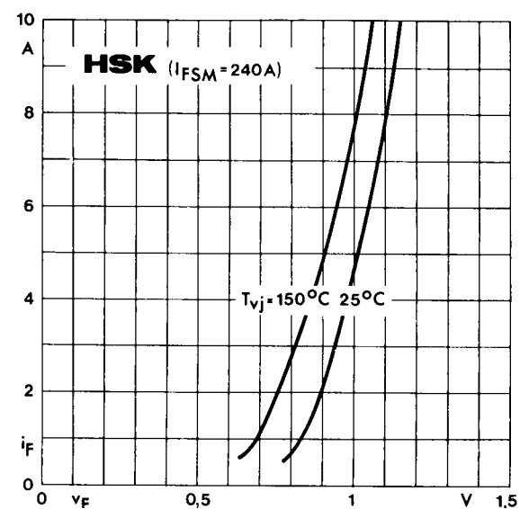
Fig. 5 a Forward characteristic of a single chip
